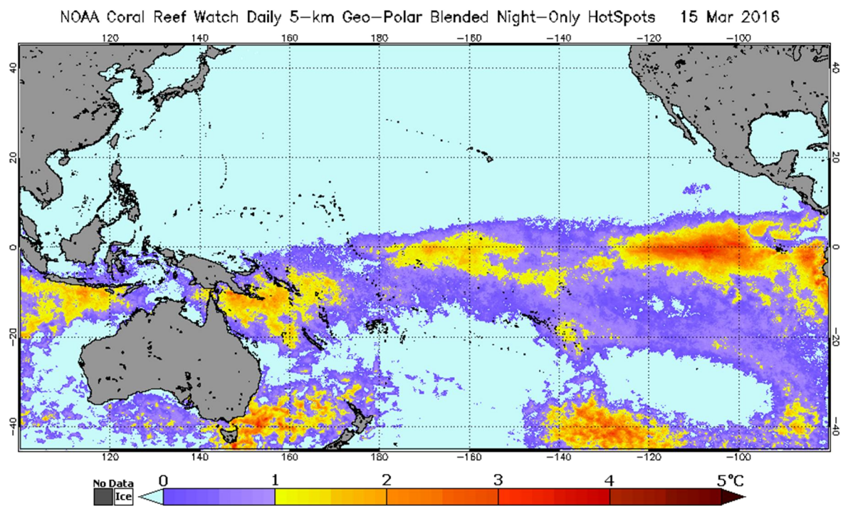
Figure 5. Hotspots before (1 February 2016) and after (15 March 2016) cyclone Winston, at 5 km pixel resolution. Source: NOAA Coral Reef Watch
